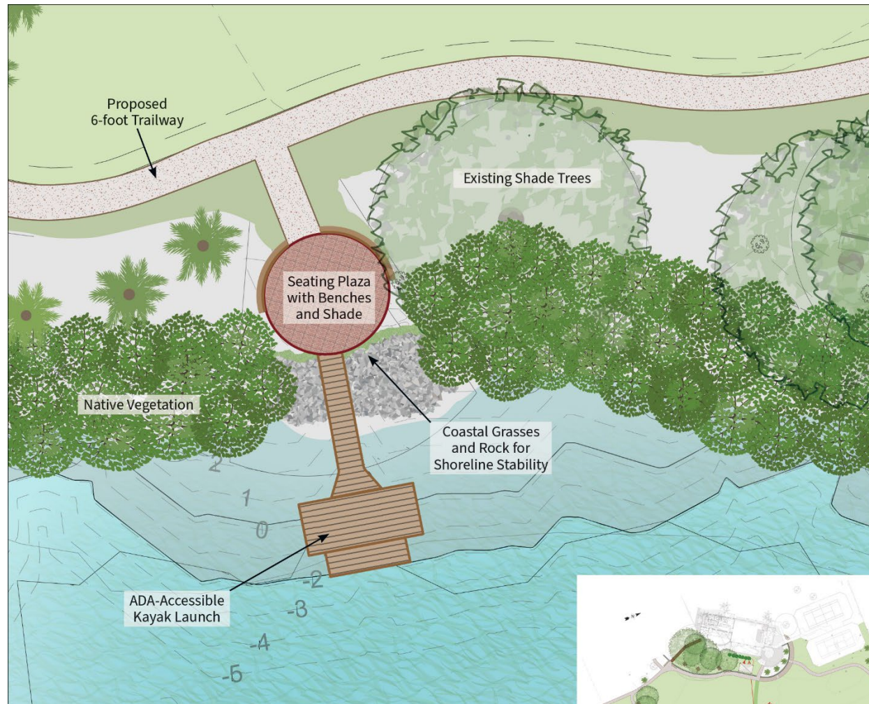
Proposed Plan for Kayak Launch at Seating Plaza with Bay View
